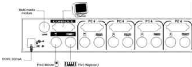
Figure 3: Master console connection
